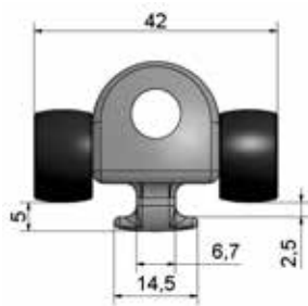
Body 16 mm 1530-16-XX
