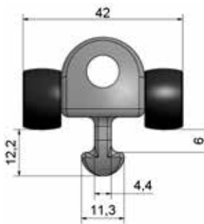
Body 11 mm 1530-11-XX & 1535-11-XX
