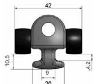
Body 20 mm 1530-20-XX & 1535-20-XX
